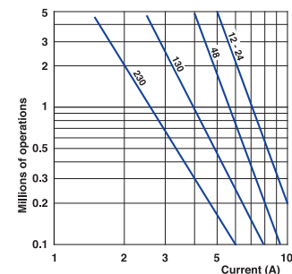
AC-15 - Slow action
