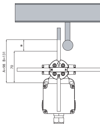
Cross and T rods
