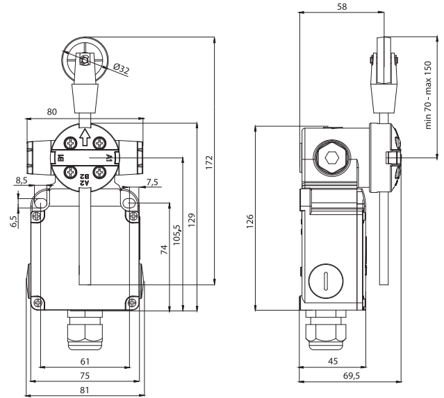
Dimensions (mm)
