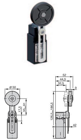
T5200 - Adjustable toothed lever (step 2 mm) with Ø 50 rubber roller
