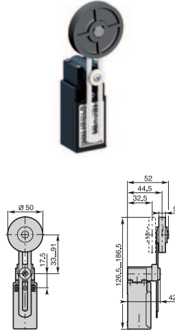
T52 - Adjustable lever with Ø 50 rubber roller
