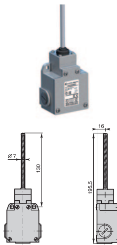
E93 - Stainless steel spring multidirectional actuator
