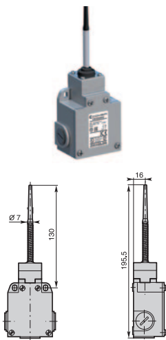
E92 - Multidirectional nylon actuator with stainless steel spring
