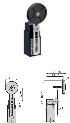
T5500 - Adjustable toothed lever (step 2 mm) with adjustable Ø 50 rubber roller
