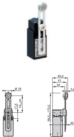
T53 - Adjustable lever with Ø 18 metal roller
