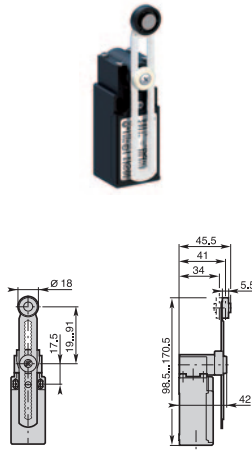
T5100 - Adjustable toothed lever (step 2 mm) with Ø 18 nylon roller
