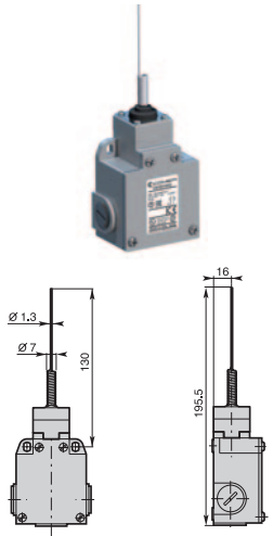
E91 - Stainless steel spring multidirectional actuator
