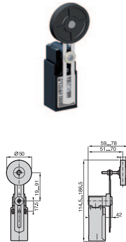
T55 - Adjustable lever with adjustable Ø 50 rubber roller
