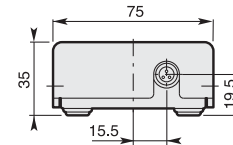
Connection by M8 connector
