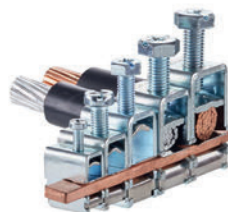
Bow terminals Page 34
