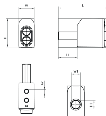
SR 2x50RB
