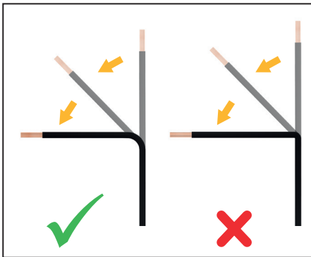
No sharp-edged bending Recommended inner radius for bending: busbar thickness 1 - 5 mm: radius 5 mm busbar thickness 6 - 10 mm: radius = thickness
