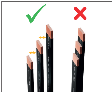
Parallel assembly has influence to heat radiation Recommended distance between bars = min. 1 x bar width. Please pay attention to correction factors for parallel assembly!
