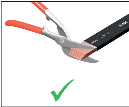
Bars must be cut if copper slides emerge after bending
