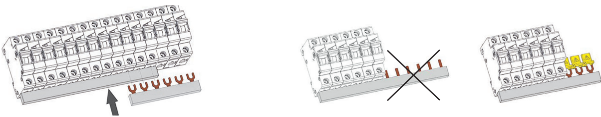
Extensions can be easily made by overlapping the busbars. For busbars with fork or pin lugs that are not required, yellow contact protection covers with a voltage warning symbol are available.
