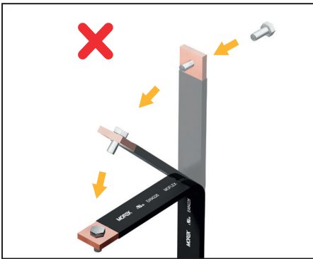
Copper files slide when bending to compensate the different length of inner and outer file No fixation before bending! It hinders the slide and may lead to burst of PVC-coating.
