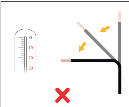
No bending at low temperatures (< 0°C or < 30F) Elongation of the coating before breakage is reduced at low temperatures. Recommended is bending at room temperature.
