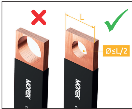
Do not drill holes exceeding half of the width of the bar
