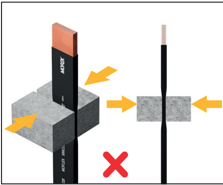
Please avoid crushing of the PVC coating Damage of coating or reduced wall thickness endangers function of isolation.
