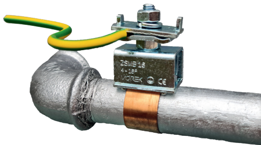
Example of application ZSMB earthing terminal
